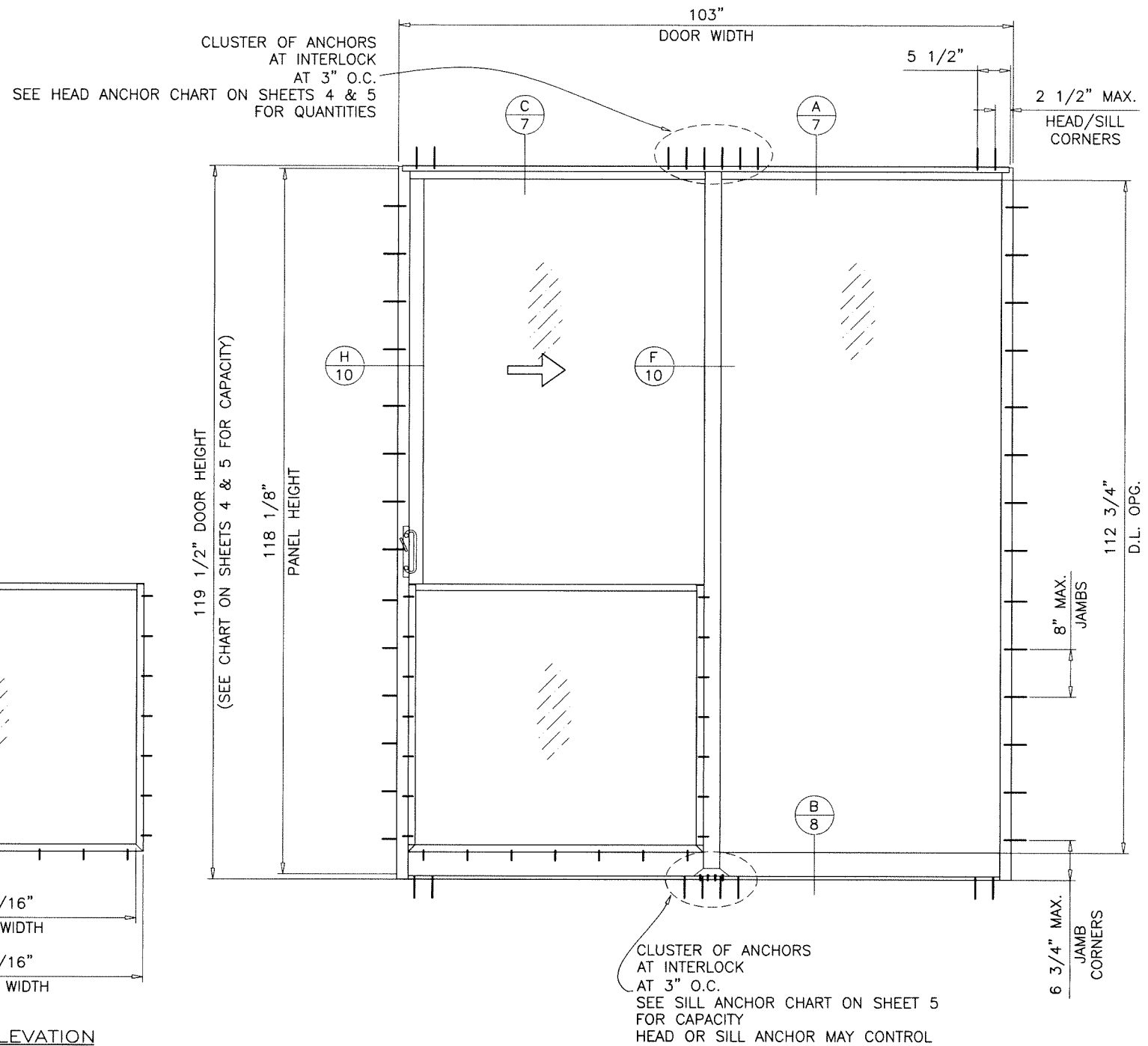
TYPICAL ELEVATION TESTED UNIT (XO WITH RAILING)
