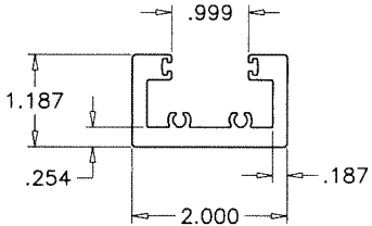
2R RAILING BOTTOM/SIDE FRAME
